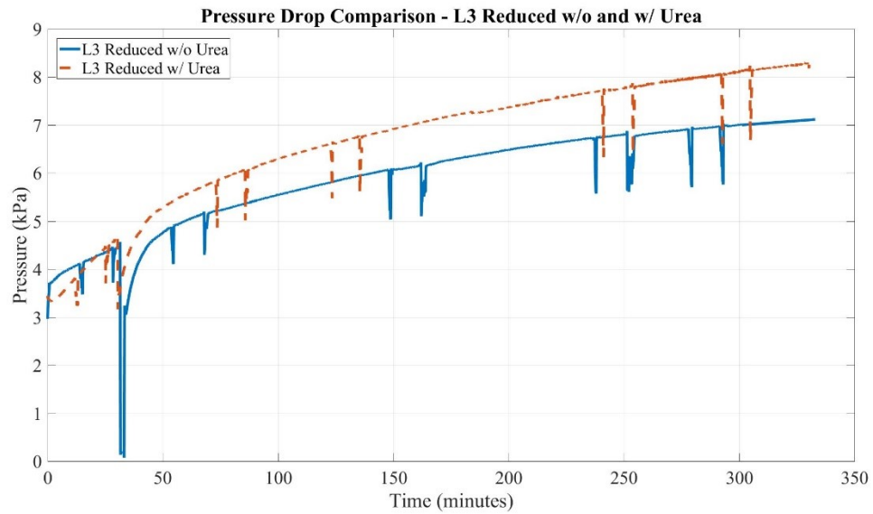
Figure C.12: SCR ® Pressure Drop Comparison for L3 Reduced w/o and w/ Urea
