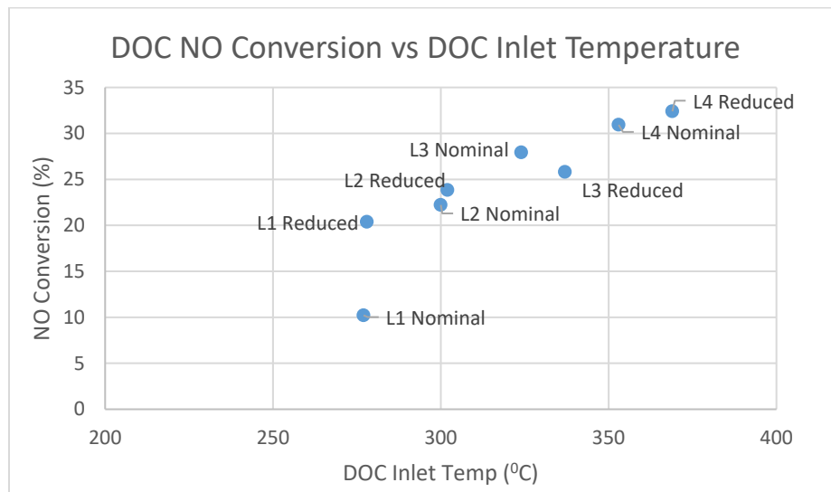
Figure 5.1: NO Conversion Across DOC vs DOC Inlet Temperature for Loading Tests w/o Urea
