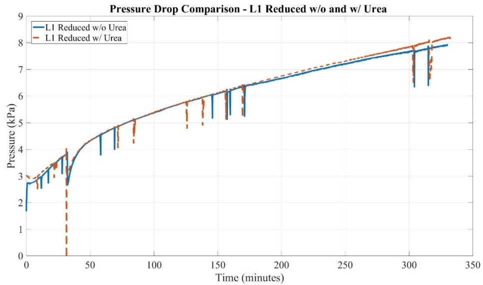
Figure C.10: SCRF® Pressure Drop Comparison for L1 Reduced w/o and w/ Urea
